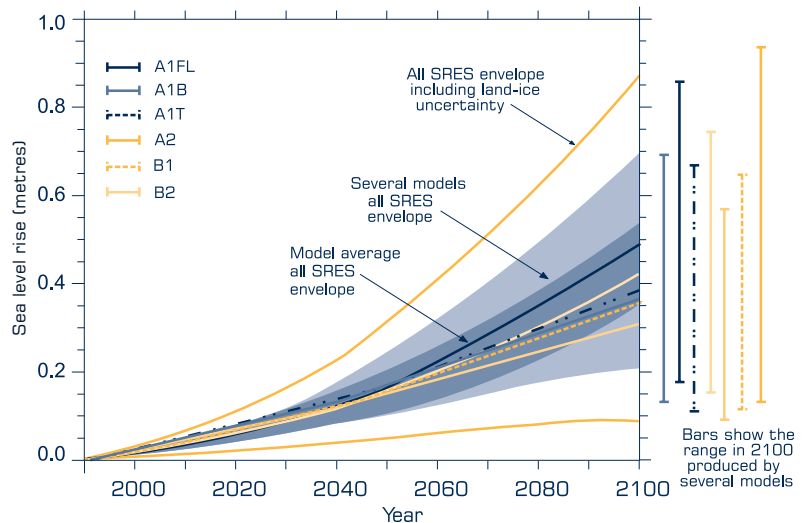
(b) Sea level rise
