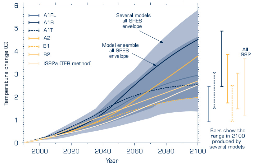
(a) Temperature change
